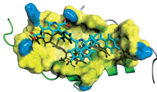
Figure 4. Model of the interaction between terpyridine 1b (cyan) and the D/D domain of human regulatory RII \alpha subunits of PKA. The primary structure of the D/D domain is SHIQIPPGLTELLQGYT-VEVLRQQPPDLVEFAVEYFTRLREAR (gene bank entry accession NP_004148); the residues of the pocket are shown with side chains and a translucent surface (yellow: hydrophobic, blue: hydrophilic). The binding pocket is rather hydrophobic (I5, P6, L9, T10, L13, T17, L21) and contains the possible hydrogen-bond donors Q4 and Q14 at the rim (blue); Q4 and Q14 are predicted to interact with the carboxy groups of the terpyridine moiety of 1b . For details see the Supporting Information.
