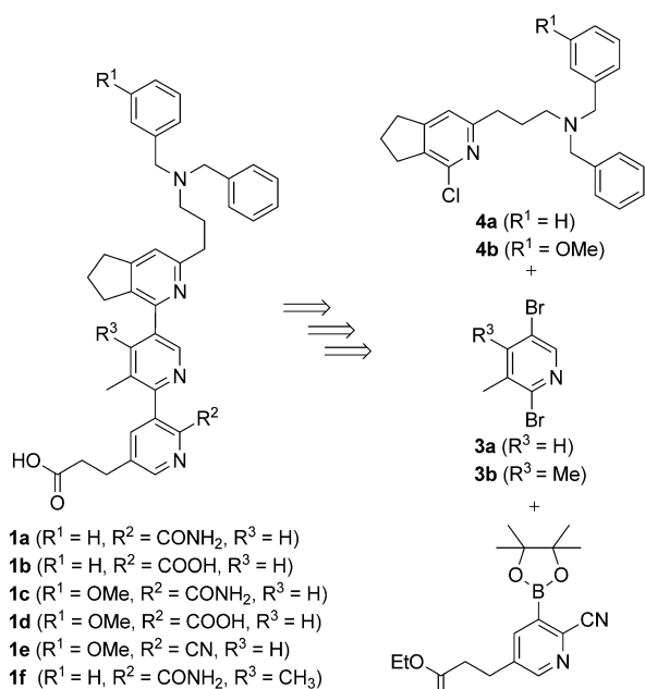
Scheme 1. Planned synthesis of terpyridines 1a–f by a sequence of Suzuki coupling reactions.
