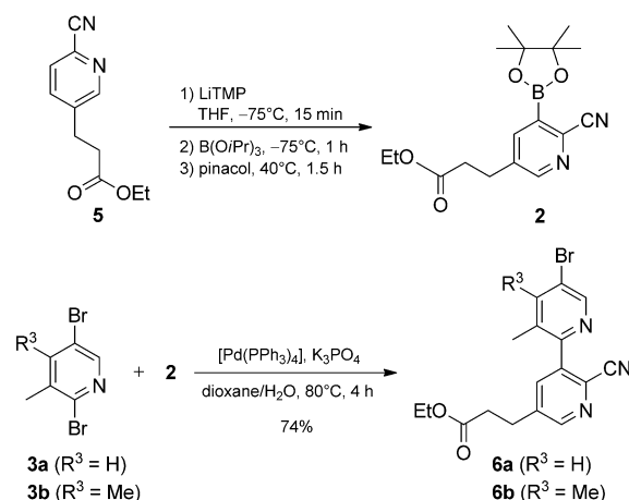
Scheme 2. Synthesis of bipyridyl bromides 6a,b , the building blocks for the final coupling reaction. TMP = 2,2,6,6-tetramethylpiperidine.
